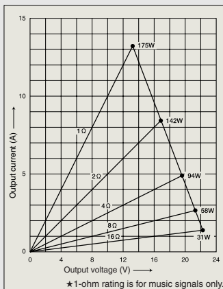
Fig. 2 Load impedance vs. output power (Output voltage/output current)
